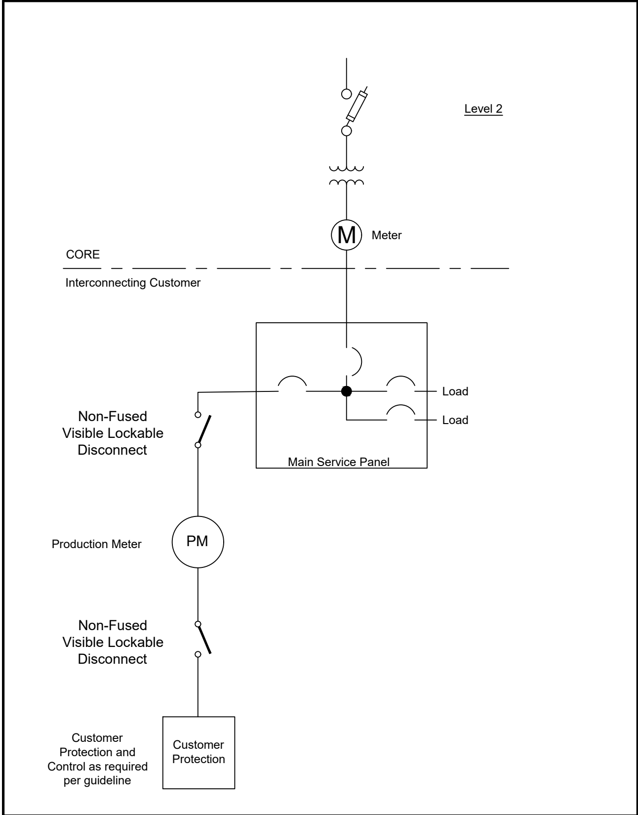
Example Level 2 Production Meter (Required) One Line Diagram
