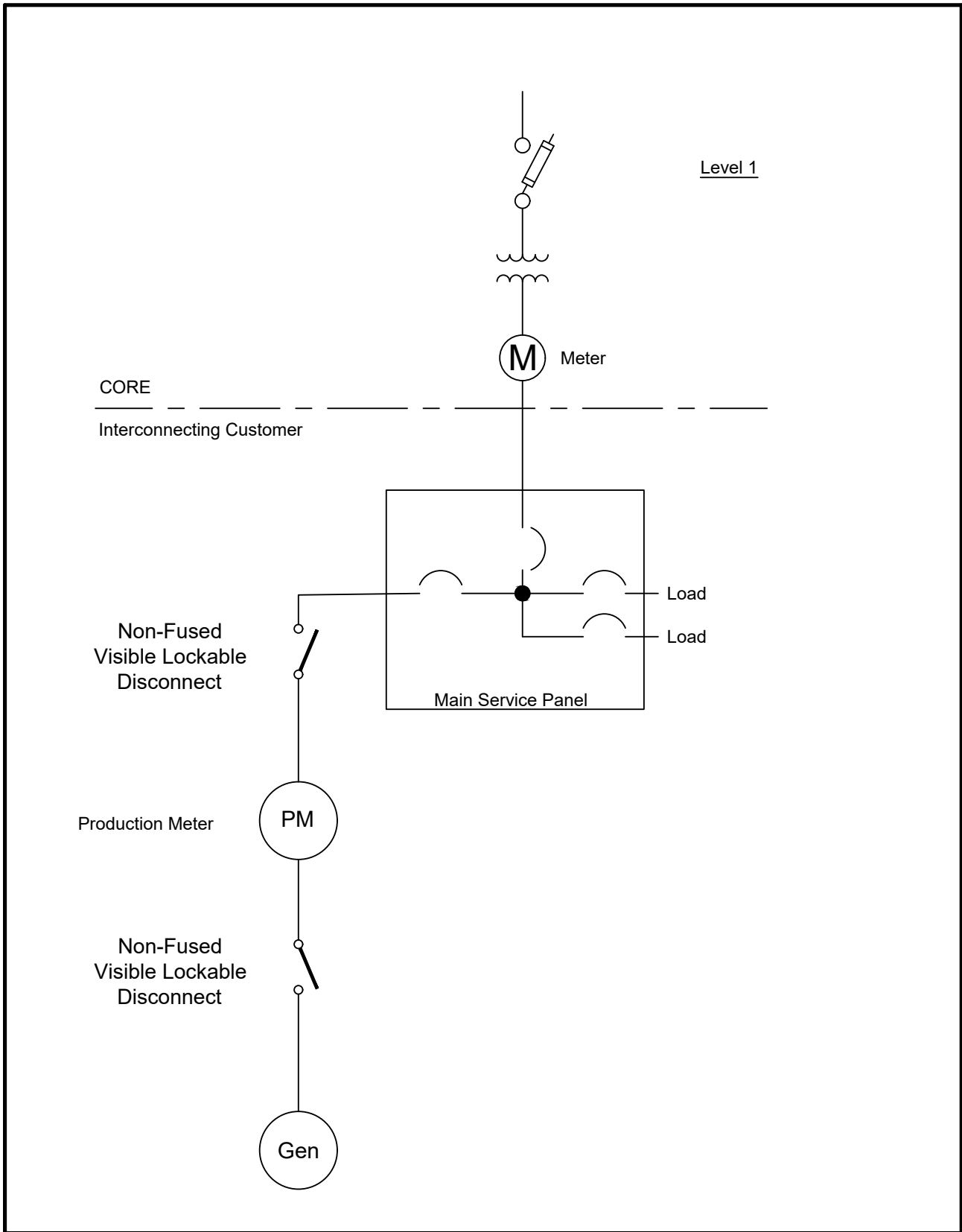
Example Level 1 Net-Metered Production Meter (Optional) One Line Diagram
